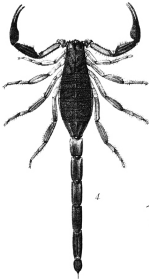
1,1a CENTRUROIDES LIMBATUS. 2,2a " " NIGRESCENS. 3,3a " " "
