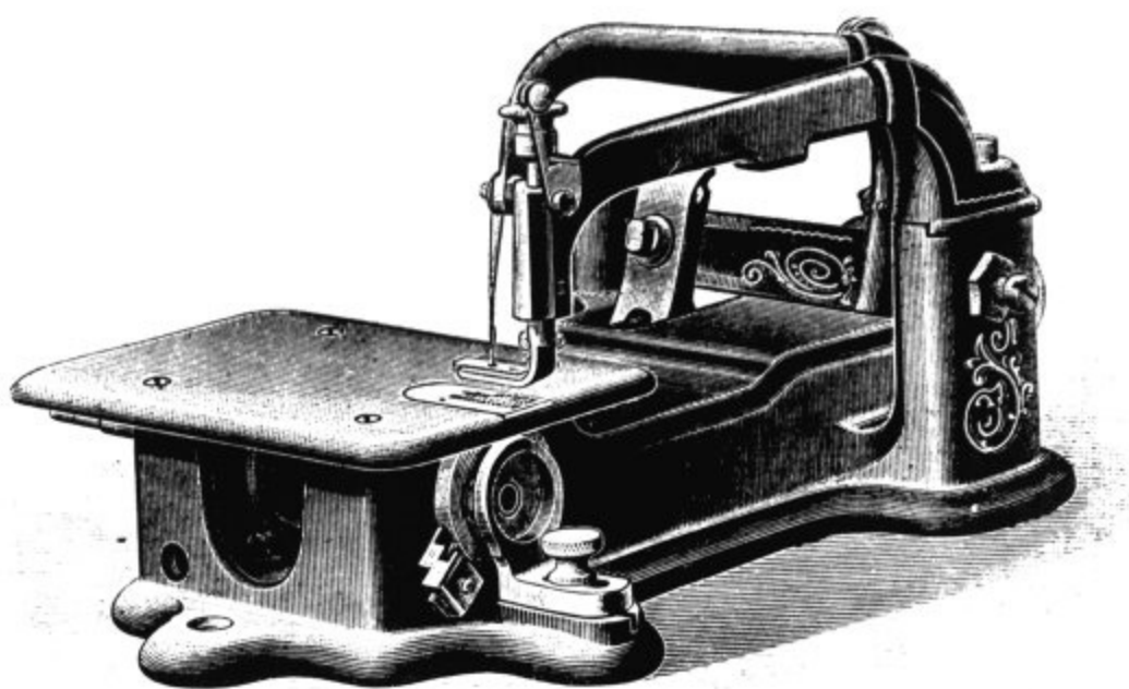
Figure 207.—SINGER SEWING MACHINE, 1924, manufacturing-machine class 1W, curved needle, is basically the Wheeler & Wilson sewing machine as manufactured by the Singer Company in the 1920s. It was designated "for fine lock stitching in the manufacture of shirts, collars, cuffs, etc." The machine head looks very much as it did in the 1860s. (Smithsonian photo 74-2123.)
