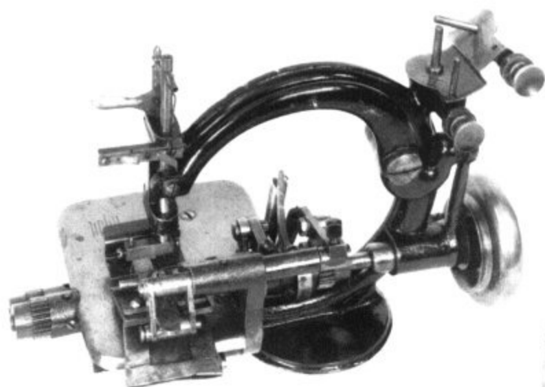
Figure 209.—WILLCOX & GIBBS FACTORY MACHINE for pleating and ruffling of 1874. Patent No. 156,119 was issued to Samuel Barney. (Smithsonian photo 73-11196.)
