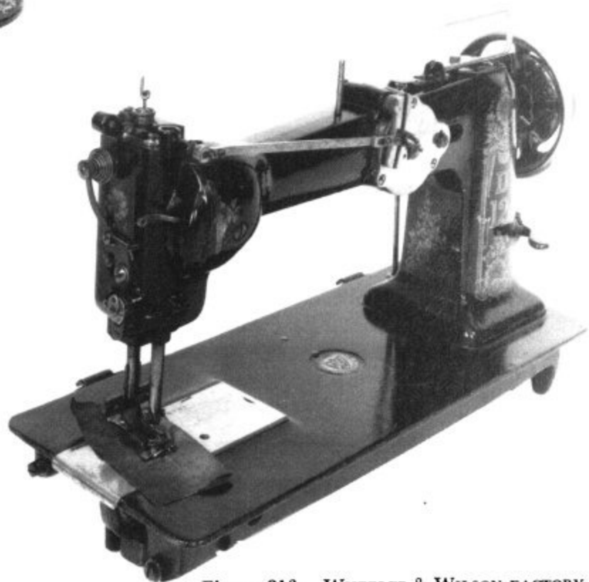
Figure 213.—WHEELER & WILSON FACTORY MACHINE of 1891 for a 3-stitch zigzag. (Smithsonian photo 73-11200.)
