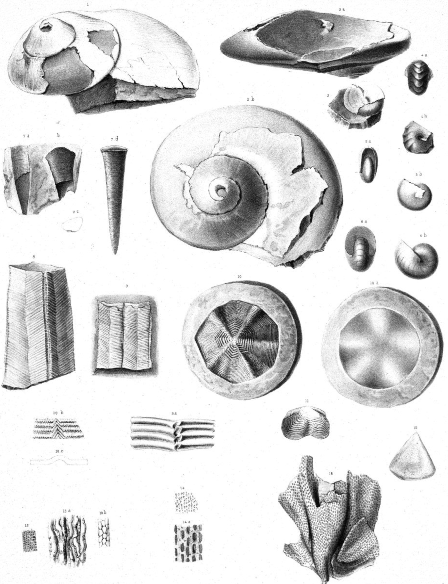
Fig. 1, Platyschisma oculus . — 2 a, b, P. depressum . — 3, Natica . — 4 a, b, Bellerophon undulatus . — 5 a, b, B. strictus . — 6 a, b, B. micromphalus . — 7 a, b, c, d, Theca lanceolata . — 8, Conularia inornata . — 9, 9 a, C. levigata . — 10, 10 a, b, c, 11, 12, Pentadia ( Tibrachyocrinus? ) corona . — 13, 13 a, b, Fenestella internata . — 14, 14 a, F. media . — 15, F. internata?
